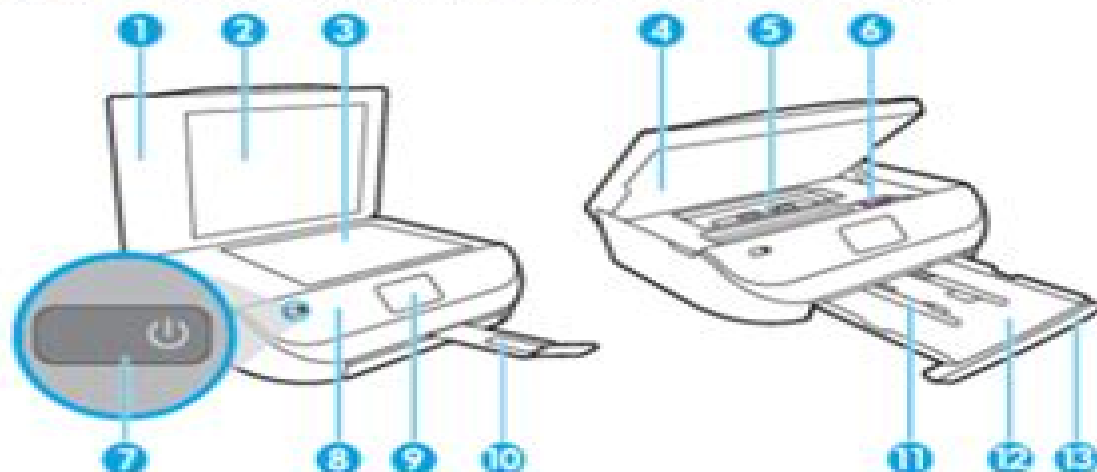
Figura 2-1 Vista frontal y superior de HP ENVY 4520 All-in-One series
