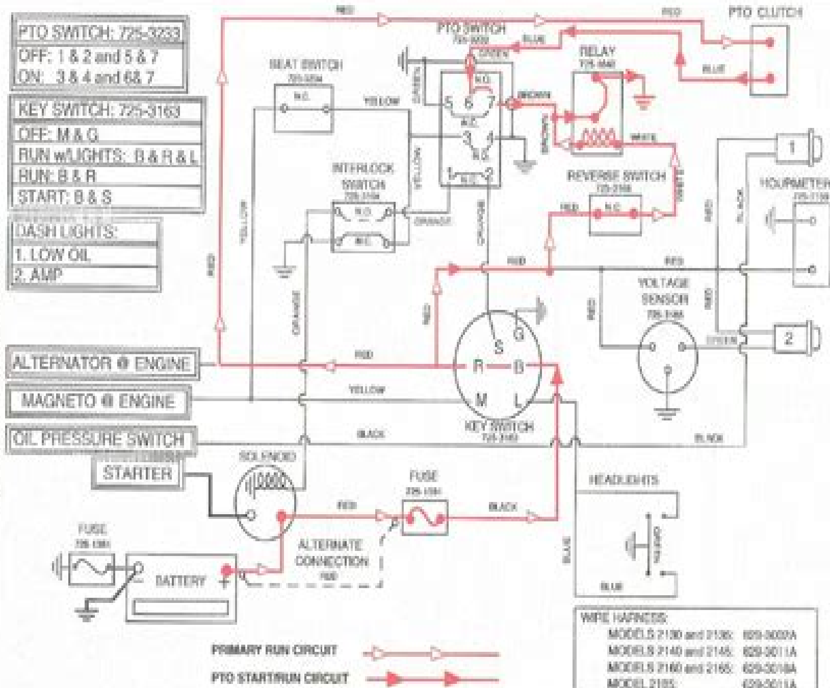
ELECTRICAL SYSTEM - PTO START
