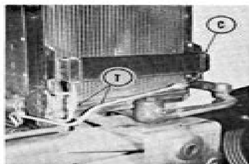
Fig. 3—Oil cooler radiator (C) can be removed after disconnecting all tubes (T).
