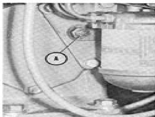
Fig. 4—Right hand view of steering gear housing showing backlash adjusting screw (A).
