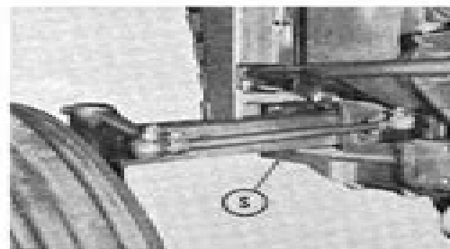
Fig. 2—On Model MF130, the cast iron front support (5) bolts to angle as shown.
