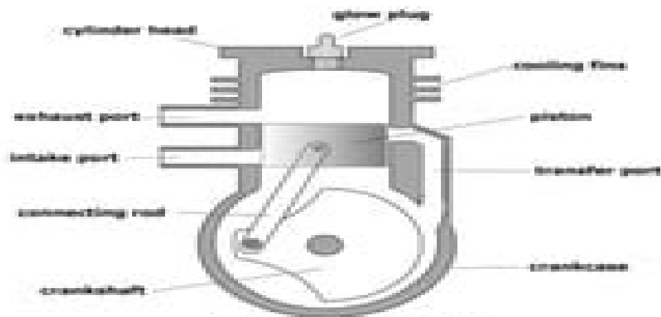
Figure: Two Stroke Engine
