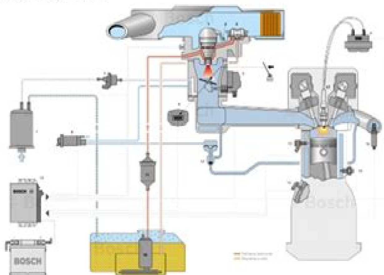
Mono-Motronic system overview
