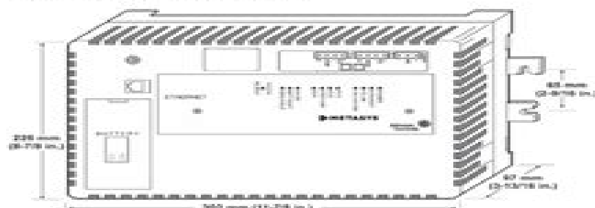
Figure 1: NAE-S Dimensions
