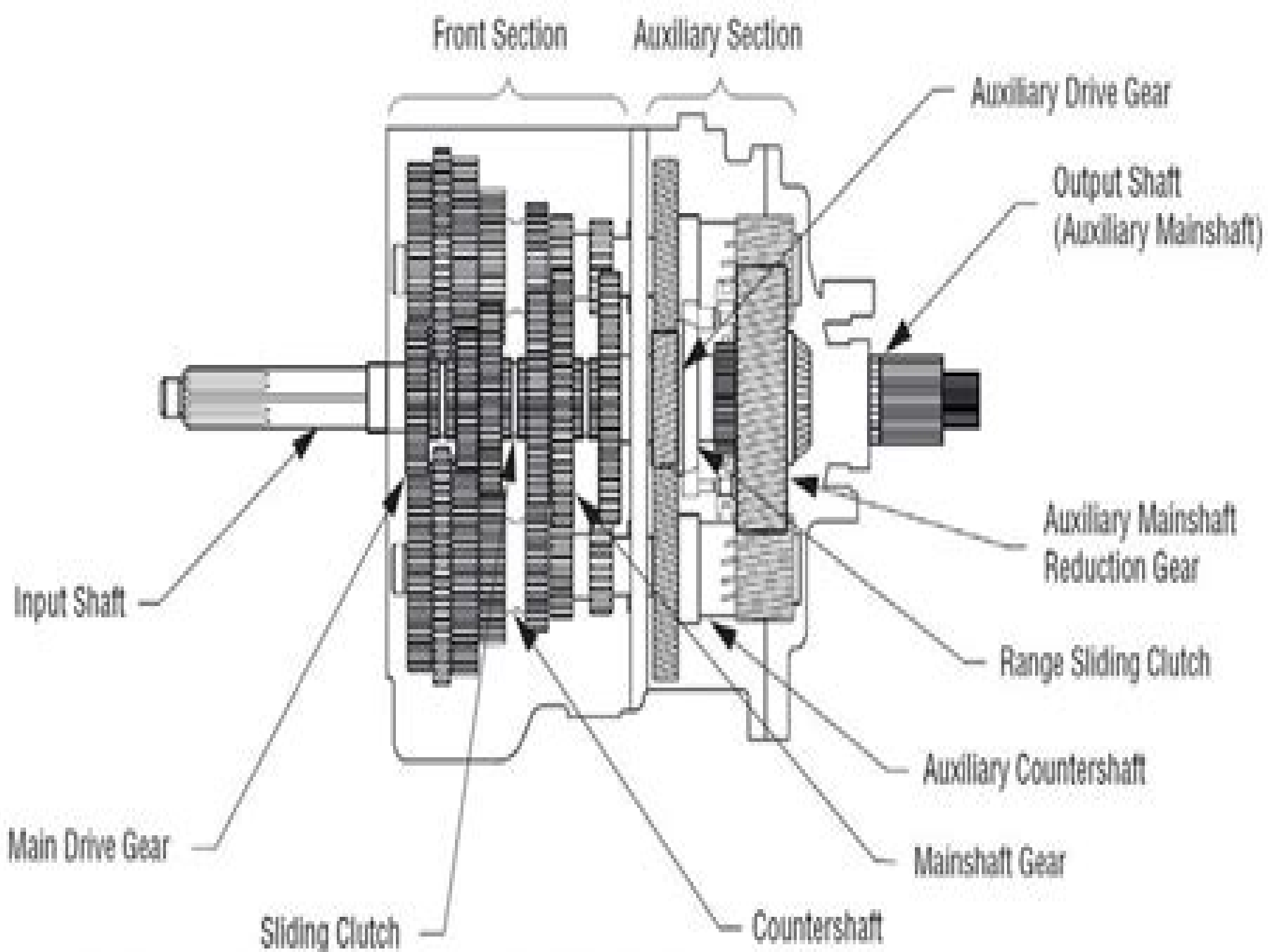
Figure 2-3. Transmission Components Important for Understanding Power Flow
