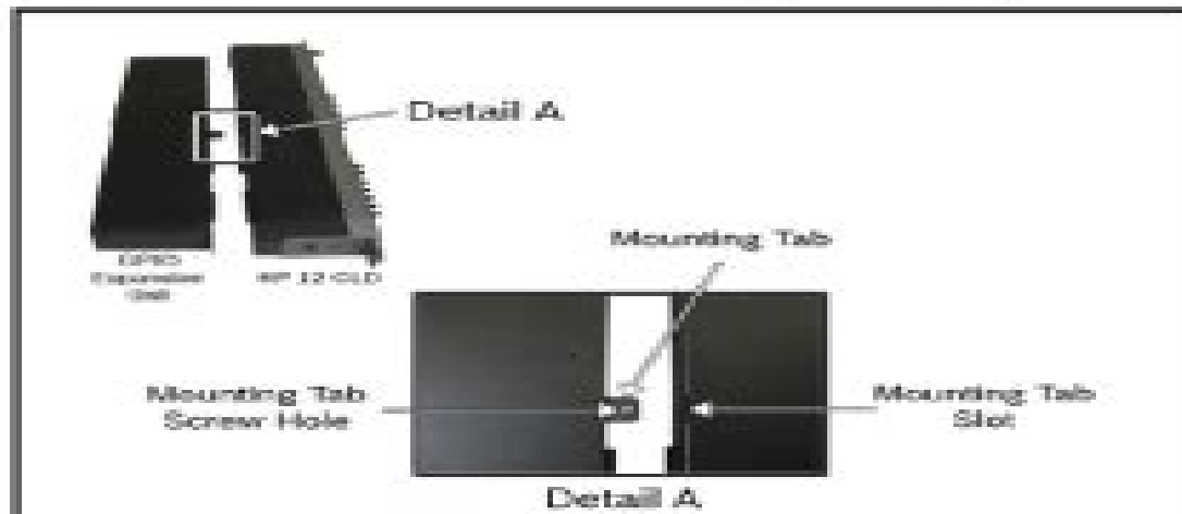
FIGURE 1. GPIO Expansion Unit — Mounting Tab Alignment with KP 12 CLD
