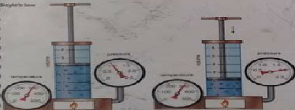
Boyle's Law
