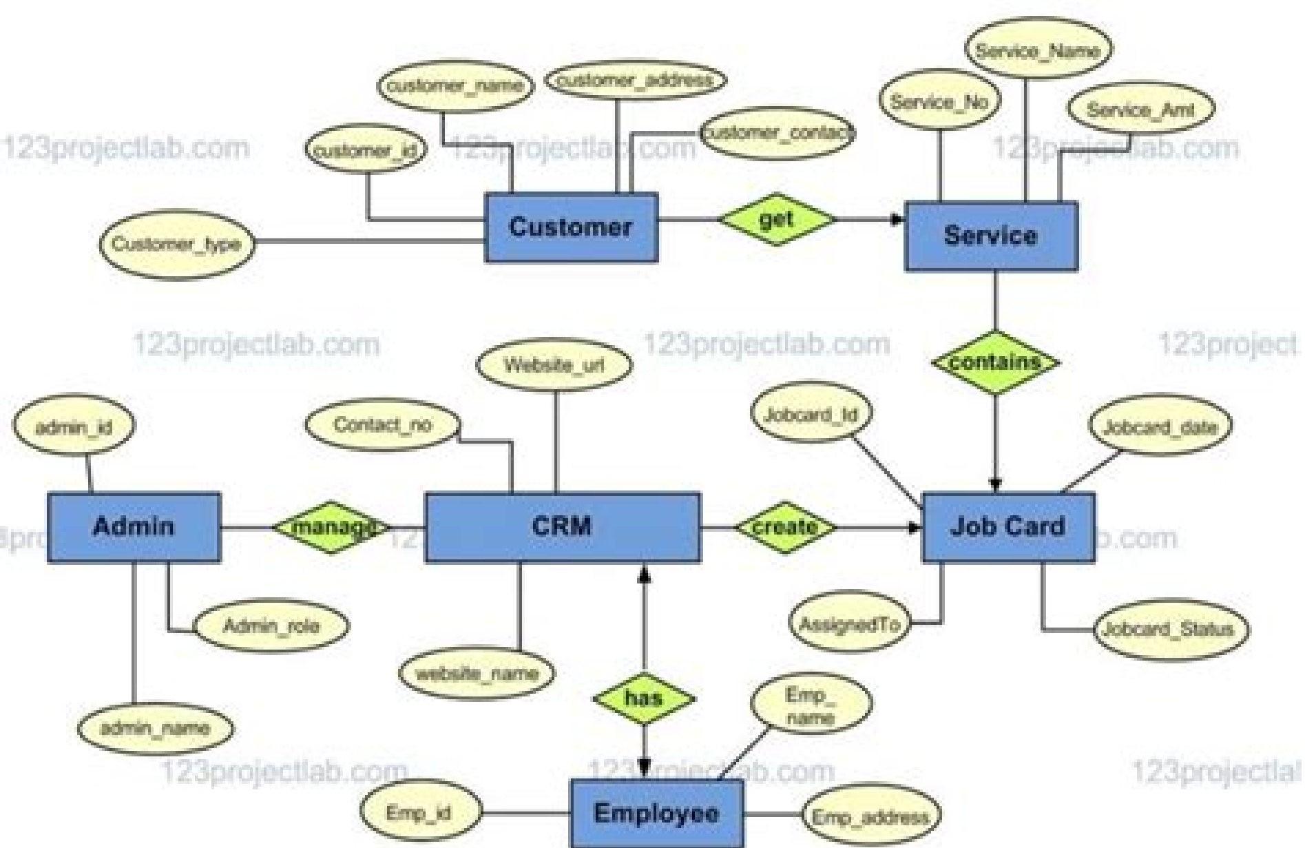
ER-Diagram for Customer Relationship Management System
