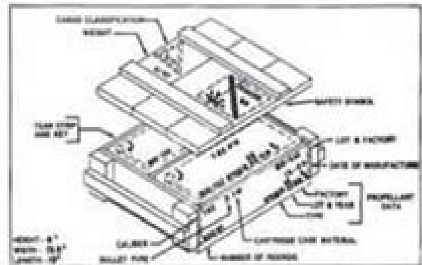
FIGURE 25. SOVIET AMMUNITION CASE
