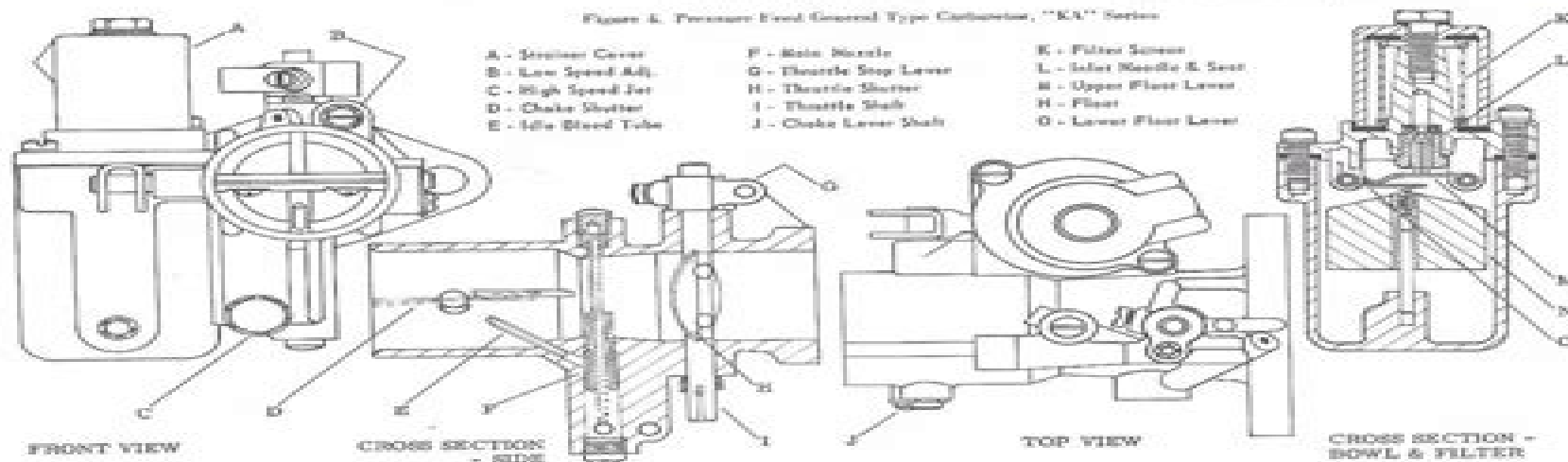
Figure 4. Pressure Feed General Type Carburetor, "KA" Series
