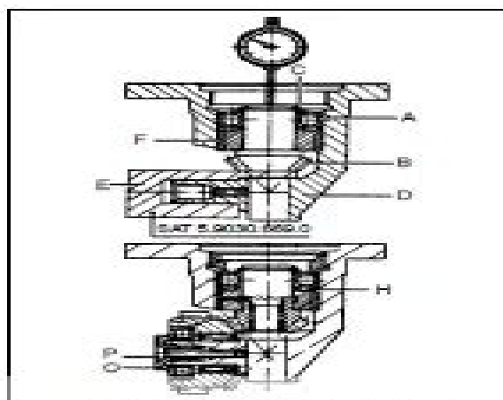
Fig. 17 - Installing pinion and crown wheel.
