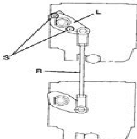
Fig. S218-8—Refer to text to synchronize carburetor throttle valves.
