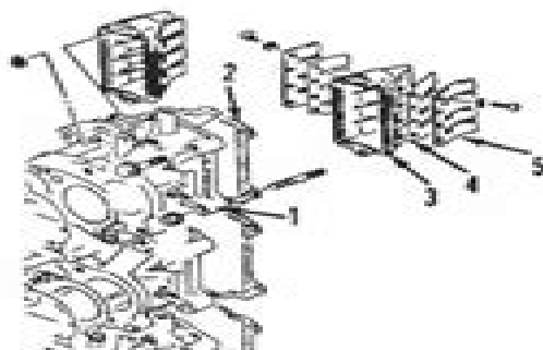
Fig. S218-6—Exploded view of intake manifold and reed valve assemblies.
