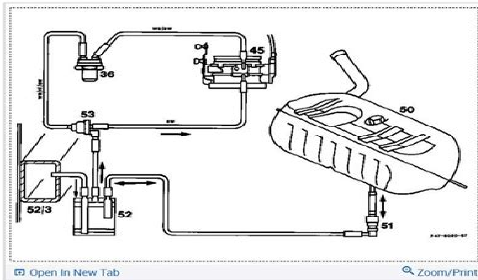
Function diagram fuel tank air admission and release, model 129
