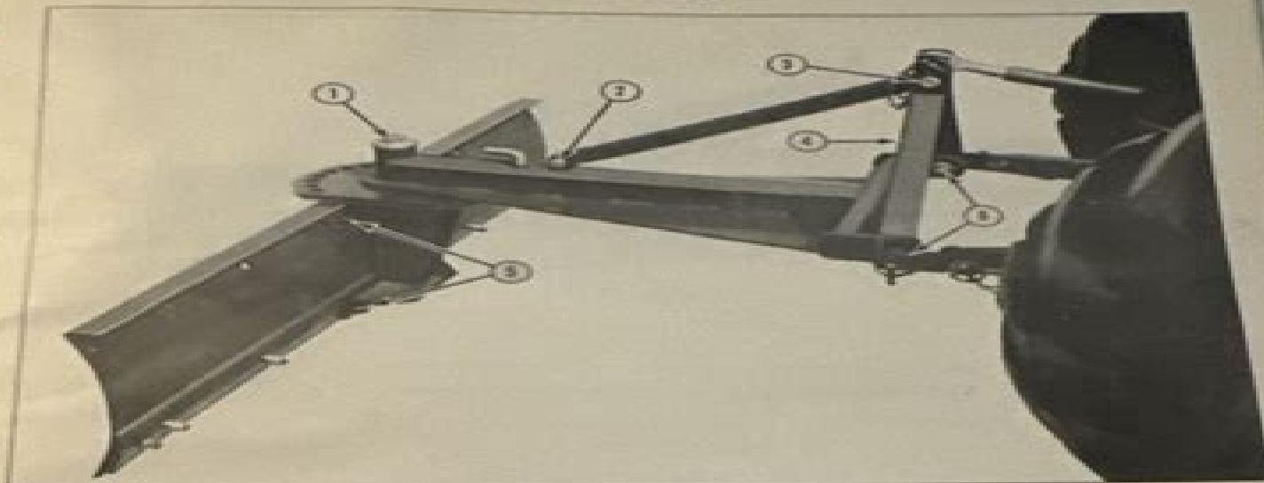
Fig. 9. Assembly of MF 16 Utility Blade
