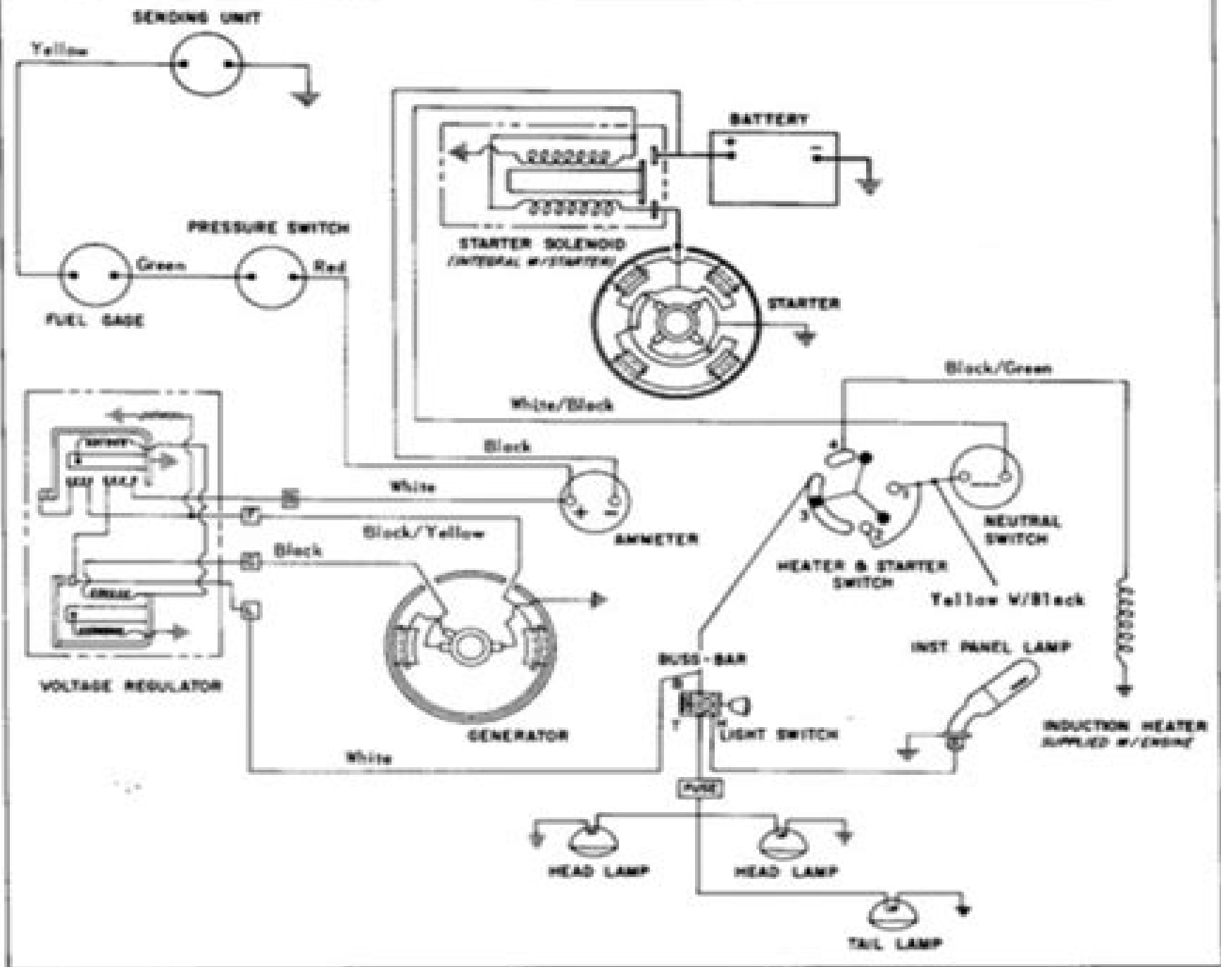
Electrical System (Diesel Tractors)
