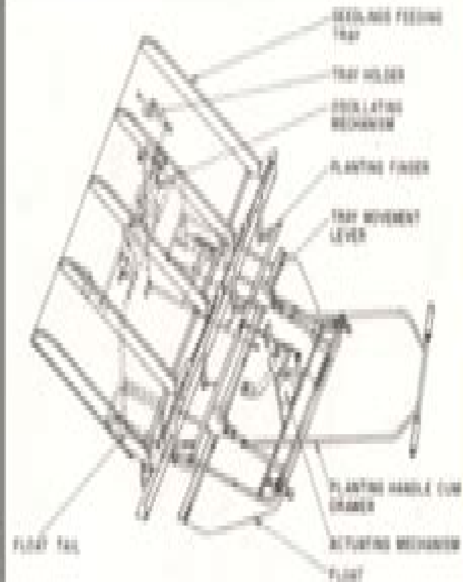
4 ROW MANUAL RICE TRANSPLANTER (MAT SEEDLINGS)
