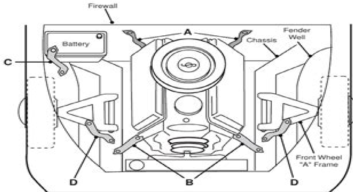
Figure 10-5. Ground Bonding
