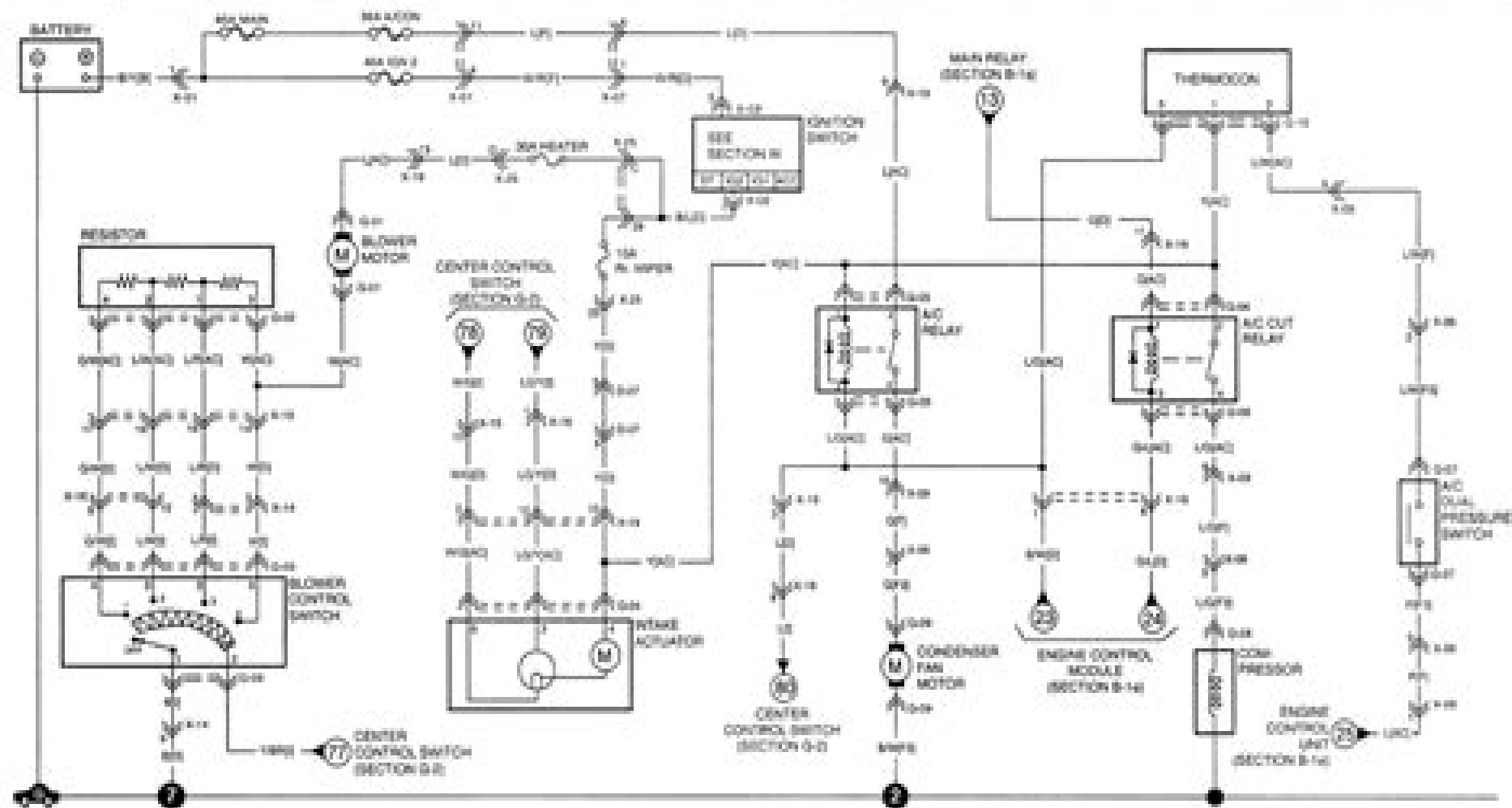
G-01 BLOWER MOTOR (AC)
