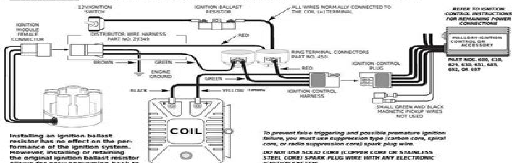
FIGURE 3 WIRING DIAGRAMS USING AFTERMARKET ELECTRONIC IGNITION CONTROLS
