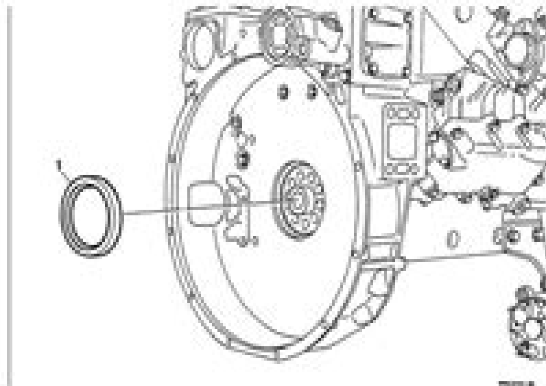
1. Radial-lip oil seal
