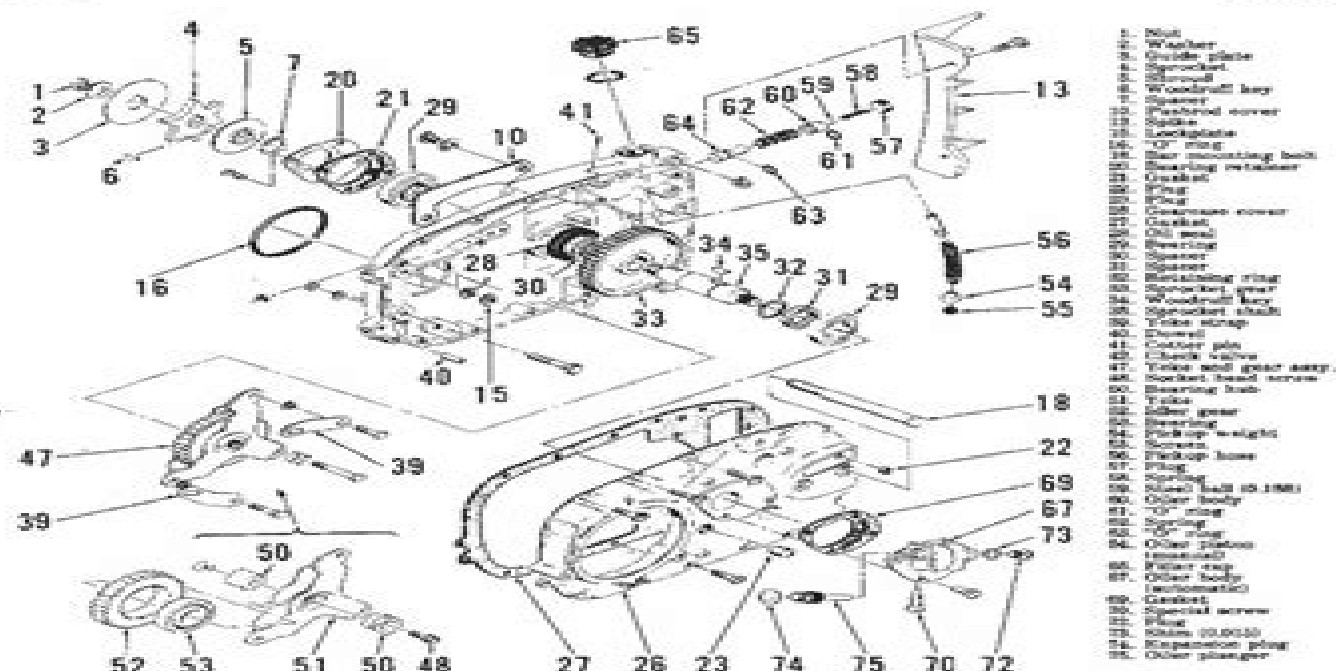
Fig. MGS-24—Exploded view of transmission used on Models 89B and 89C. Input gear is part of clutch drum (38—Fig. MGS-21). Shafts (22) are 0.015 thick.
