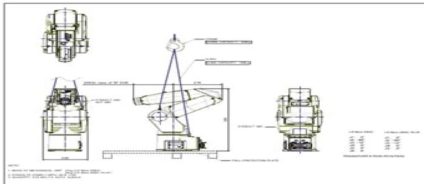
Fig. 1.1 (a) Transportation using a crane(LR Mate 200-C,LR Mate 200-C/3WP,3H,3F, ARC Mate 50-C)
