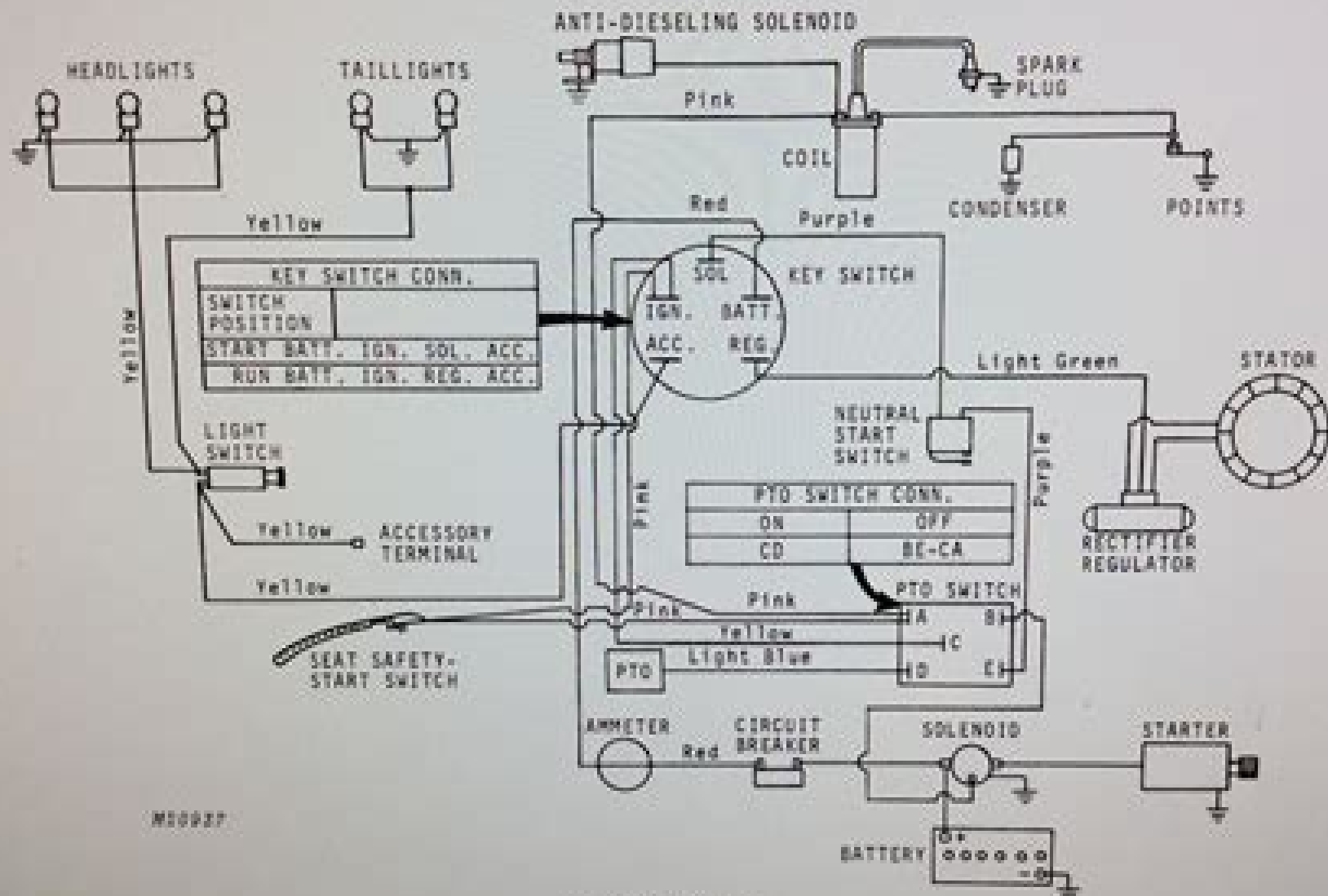
Fig. 2-Wiring Diagram
