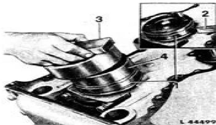
Fig. 4 — Removing Old Wear Ring - Pressing on New Wear Ring. Using Special Tools No. JD 251 and JD 251-3
