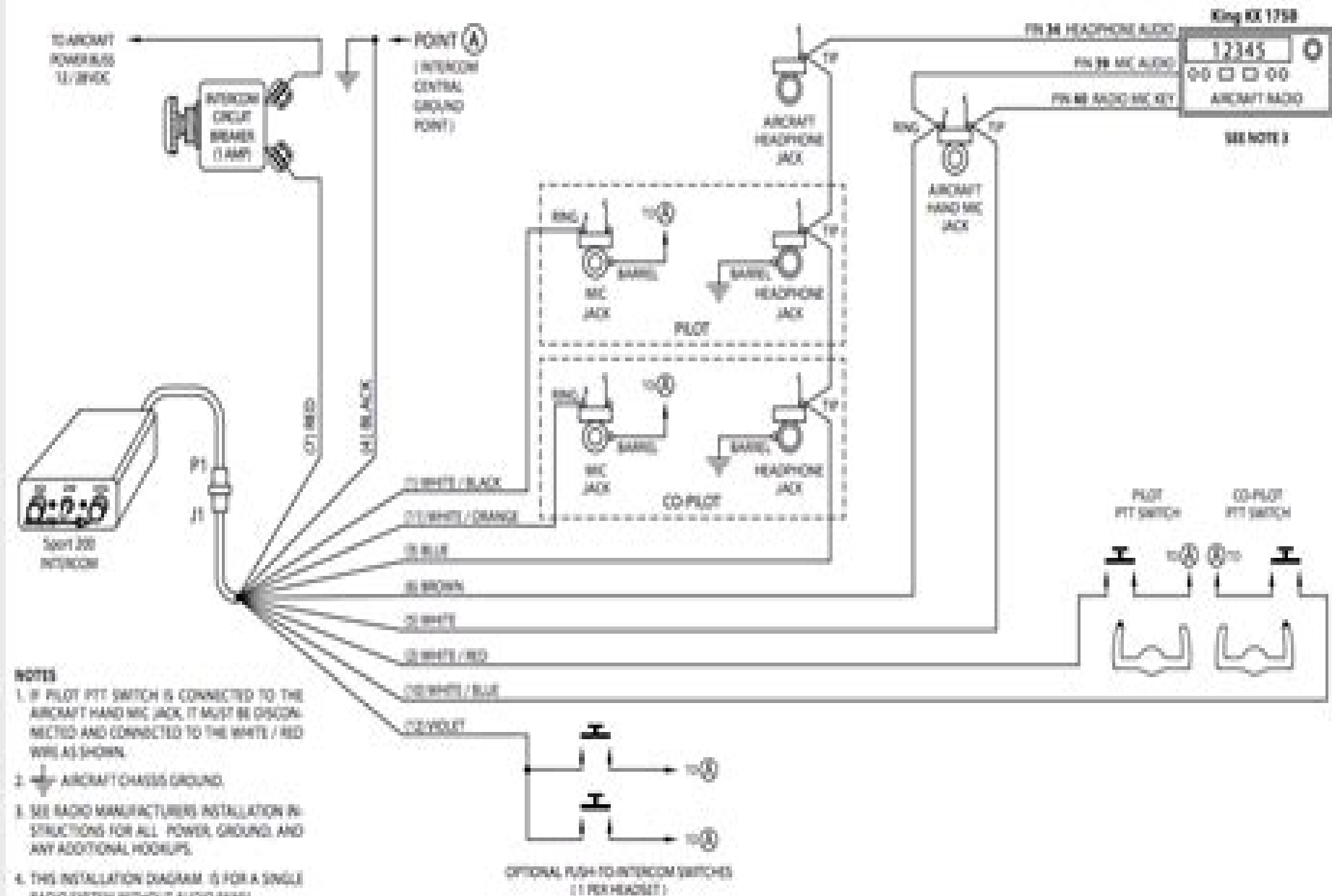
Sport 200 - King KX 175B Radio Installation Wiring Diagram
