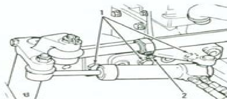
Fig. 5—View of axle left end typical of 340-360 models. Track adjusting screw and lock nut (2) and cylinder bracket and axle extension screws (1) must be properly installed and tightened.
