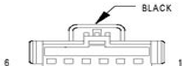
BRAKE LAMP SWITCH PINOUT
