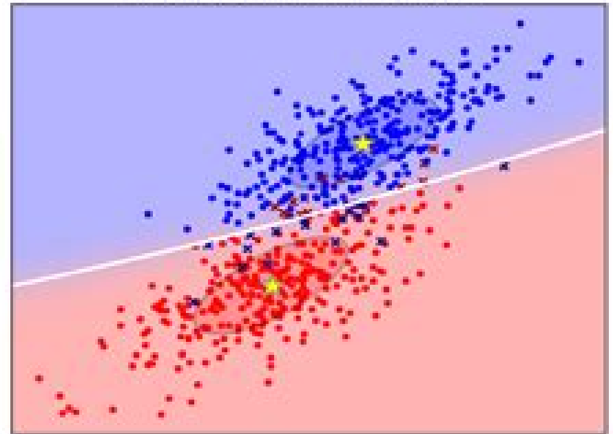
Quadratic Discriminant Analysis
