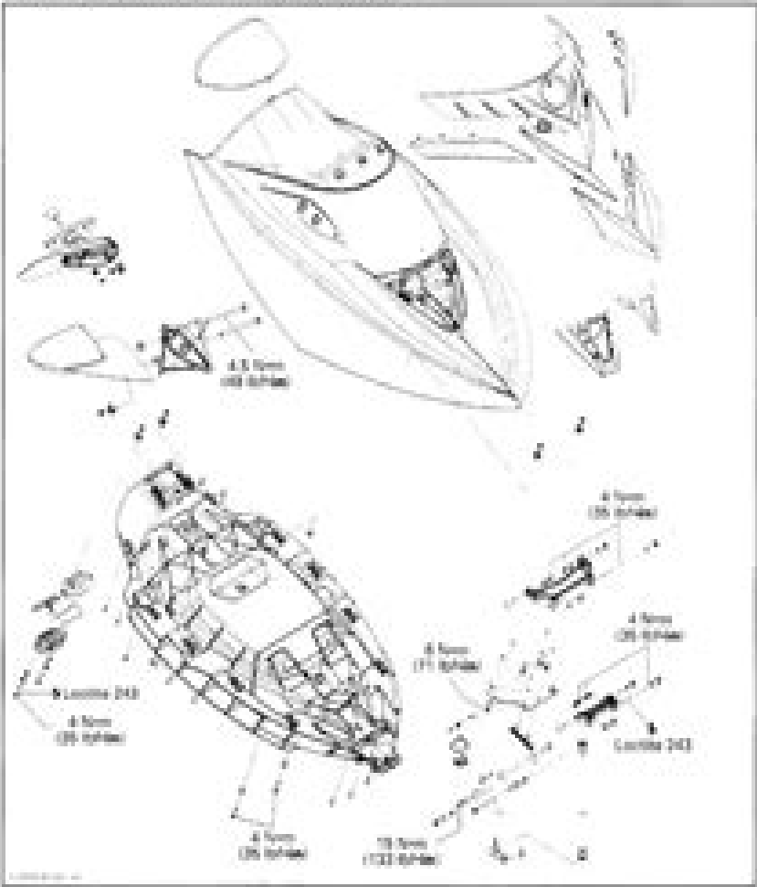
QTX Series and RXT Models (from storage compartment)
