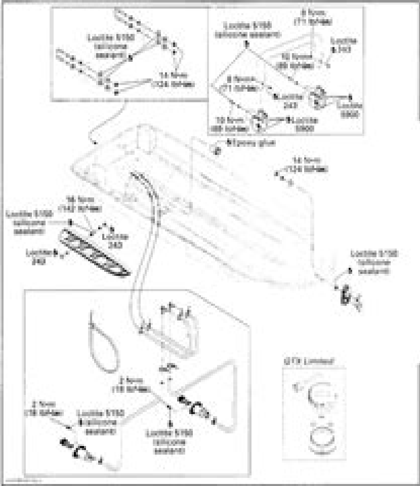
QTX Series and RXT Models (Hull)
