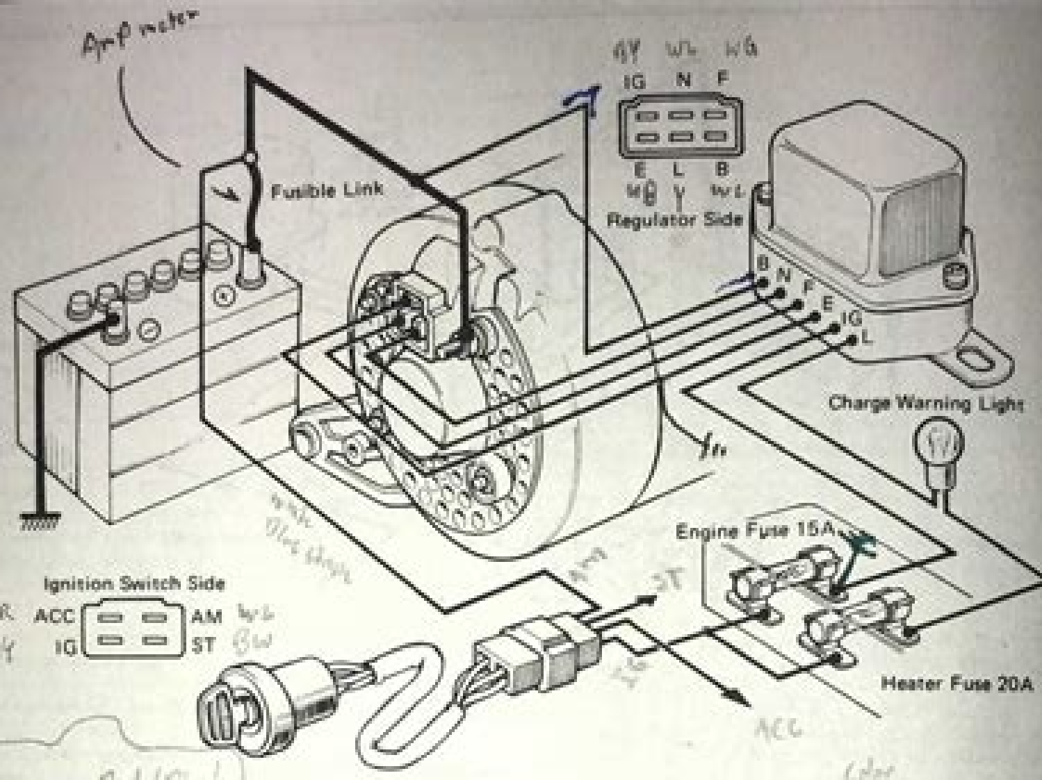
Fig. 11.2. Alternator connections - charge warning light types
