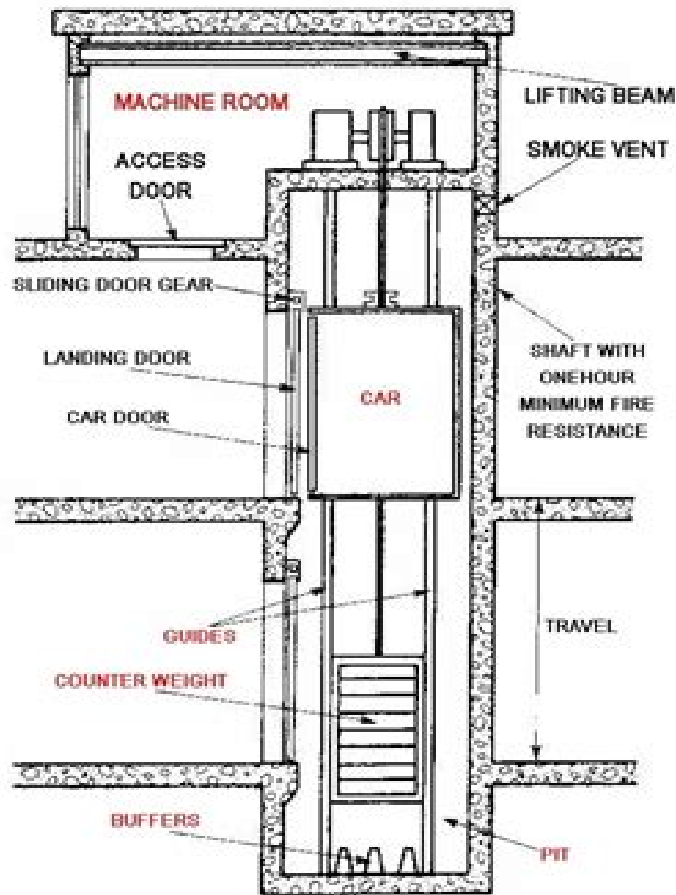
VERTICAL SECTION
