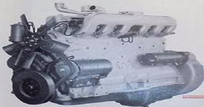
Left side of engine, showing viscous type vibration damper, generator drive, water pump, fuel oil filter, aluminum intake manifold and electric starter.
