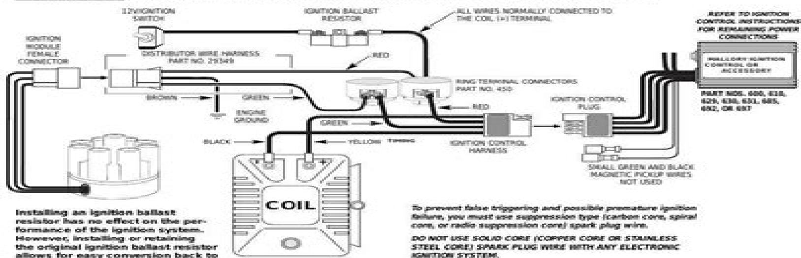
FIGURE 3 WIRING DIAGRAMS USING AFTERMARKET ELECTRONIC IGNITION CONTROLS
