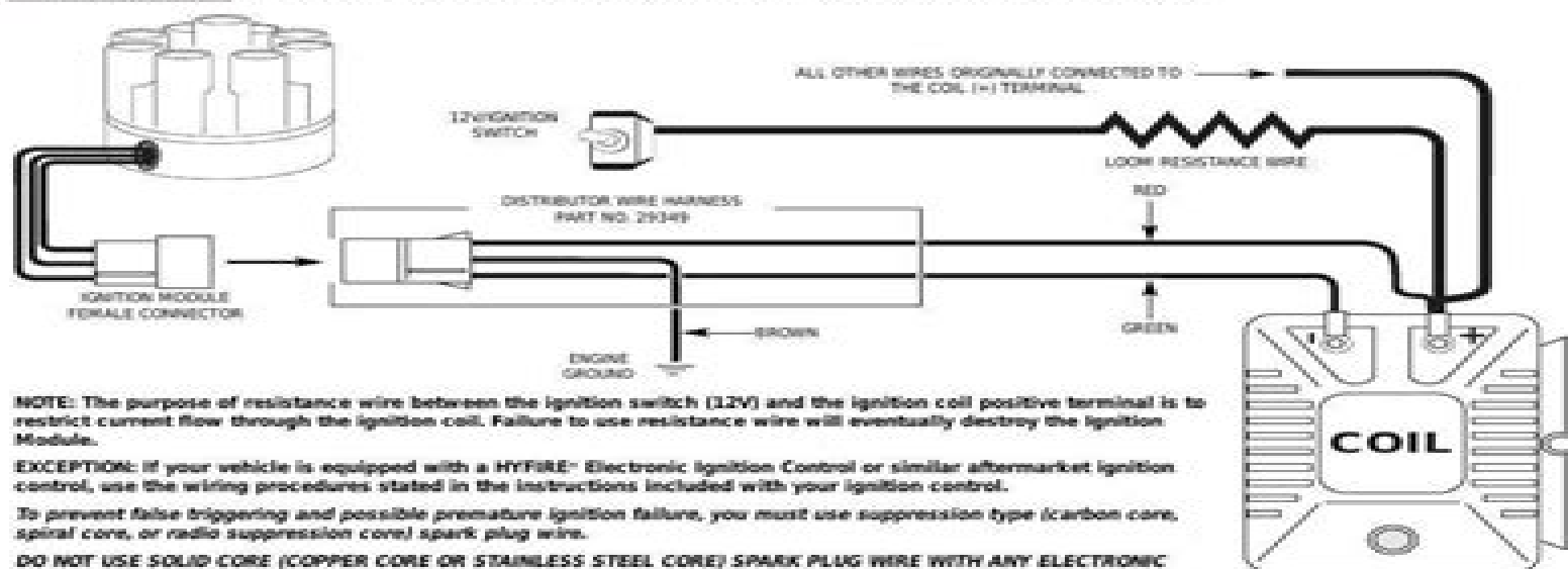
FIGURE 2 UNILITE® WIRING DIAGRAM USING OEM PRIMARY RESISTANCE WIRE
