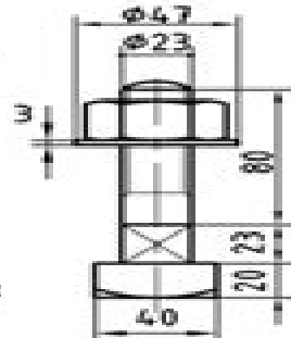
CLAMPING BOLT & NUT MS 1 OFF
