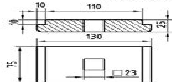
CLAMPING PLATE MS 1 OFF
