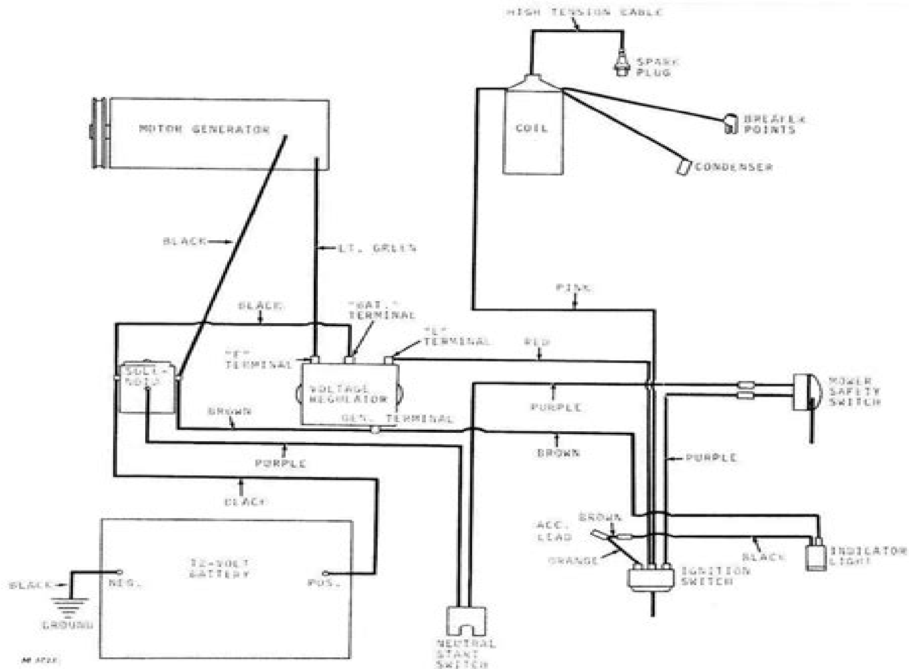
Fig. 4—Electrical System Wiring Diagram (15001).
