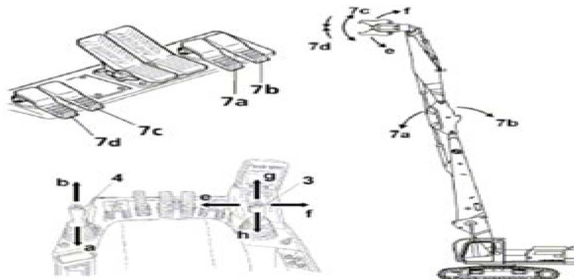
Fig. 3-82 Operating the intermediate arm and the demolition tool
