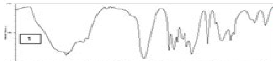
propanoic acid
