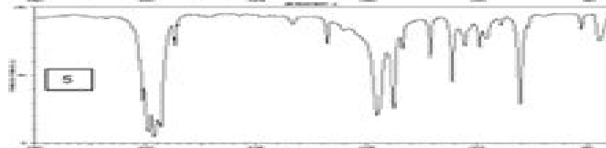
2-methylbut-2-ene
