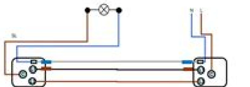
Two wire switch fed
