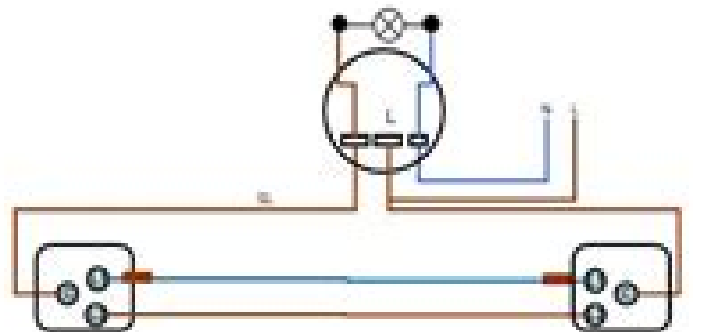
Two wire three plate
