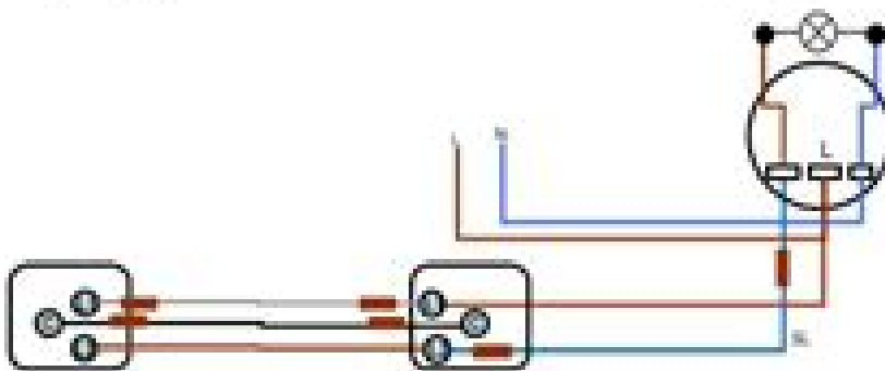
Three wire three plate
