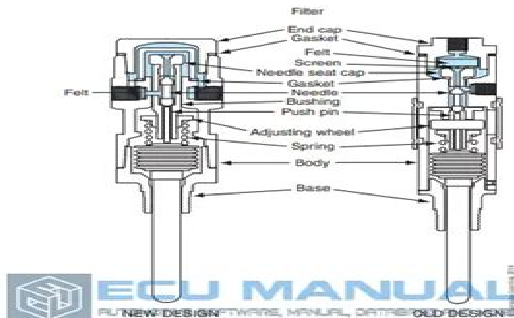
Figure 8-29 The shutterstat, which controls the opening and closing of the shutters, if equipped (cross-section view).
