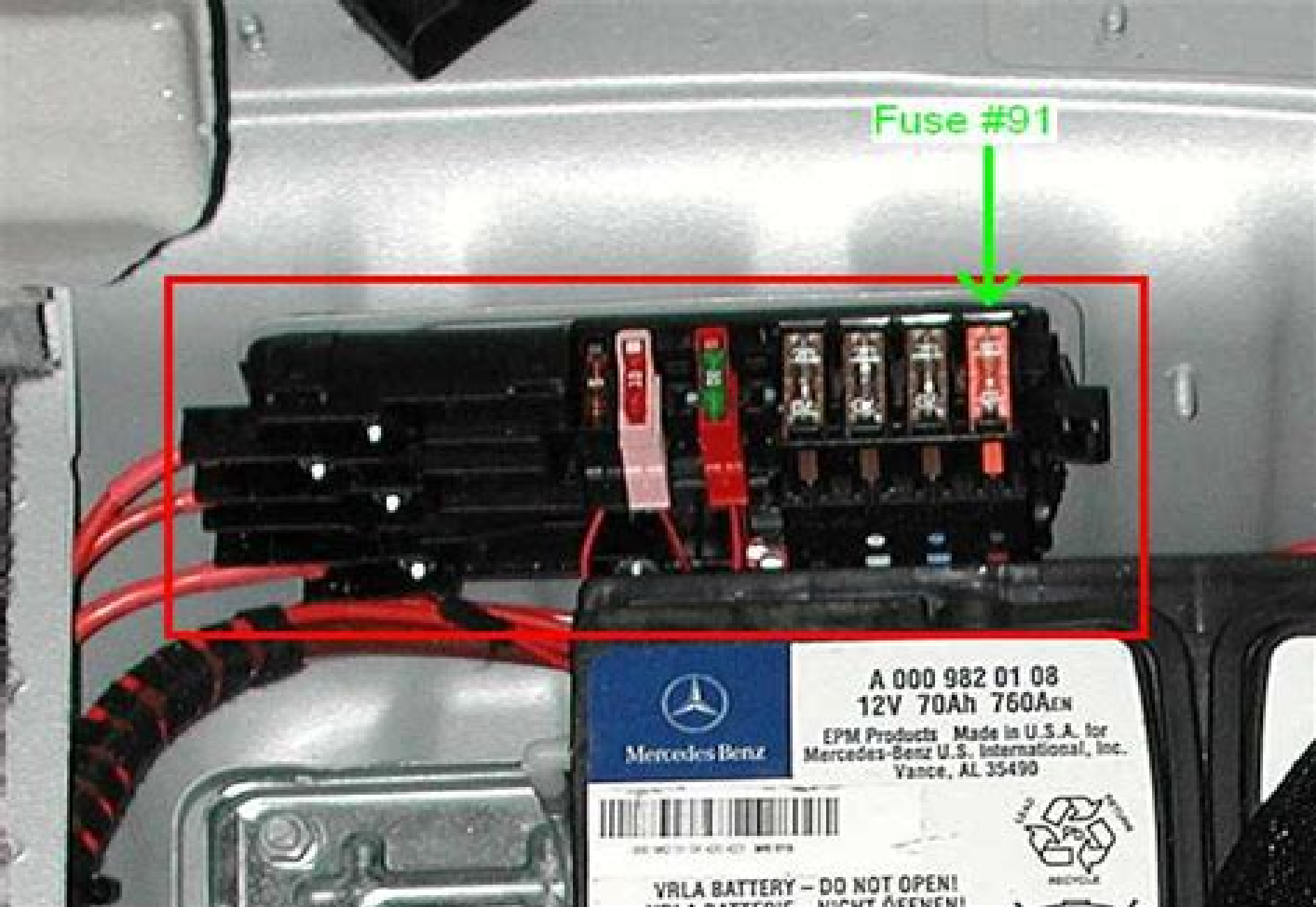
F33 Battery compartment prefuse box
