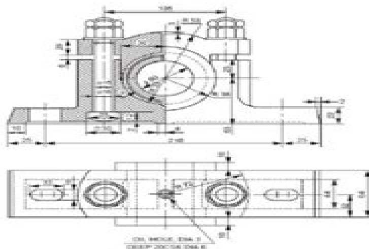
Plummer Block
