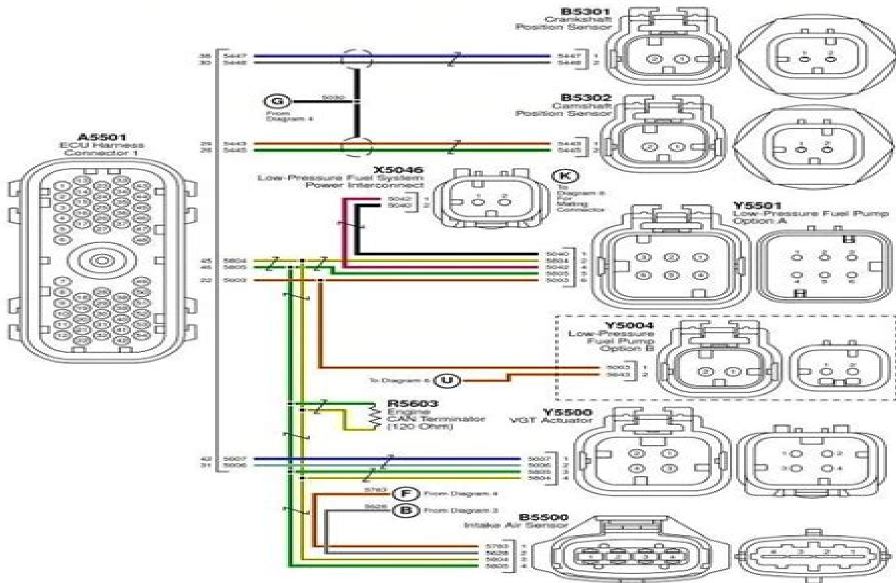
Wiring Diagram 7
