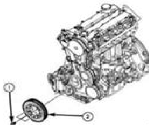
Fig. 118: Crankshaft Damper & Bolts Courtesy of CHRYSLER GROUP, LLC
