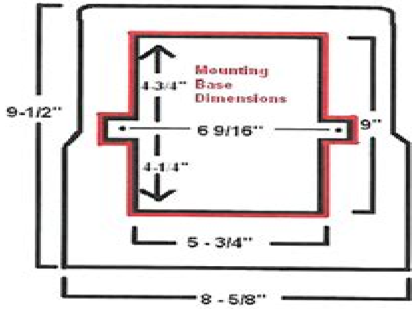
Cover Dimensions
