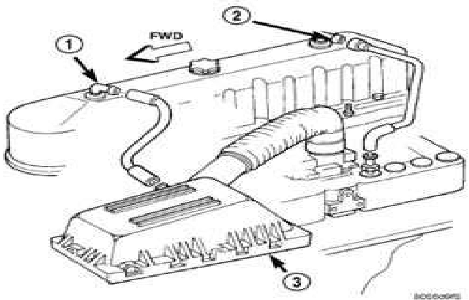
Fig. 2 CCV System—4.0L Engine—Typical
