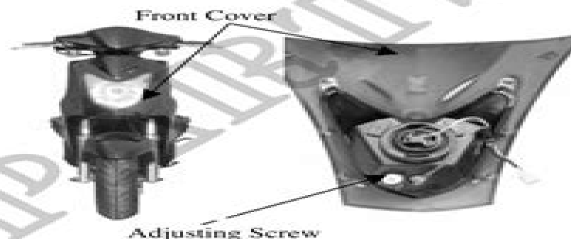
Adjusting Screw
