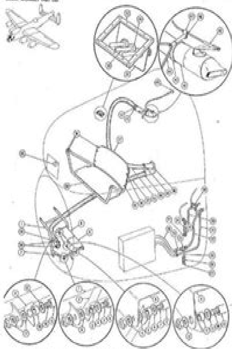
FIG. 40. ENGINE ACCESSORY UNIT, SHOWING CONNECTIONS, BELT DRIVE TO GENERATOR, FAN, AND PULLEY
