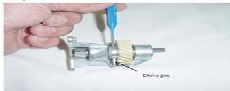
Fig. 57 The drive pin must be removed to change the gears.
